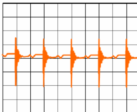
Radiation noise of conventional transformer
