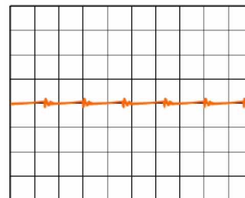
Radiation noise from spherical transformer
